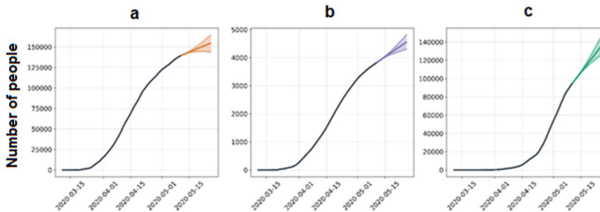
Figure B. 15-day time series prediction a) total number of cases, b) total death, c) total recovery
