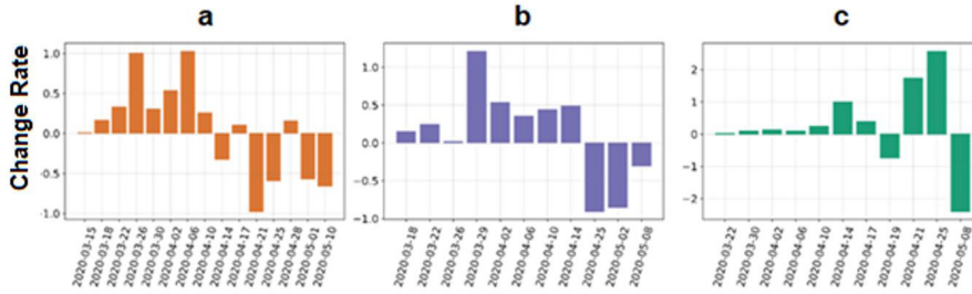
Figure-A Critical dates that show an increase or decrease in the change of data over time. a) Points of change in total case values, b) change points in total death values, c) points of change in total recovery values
